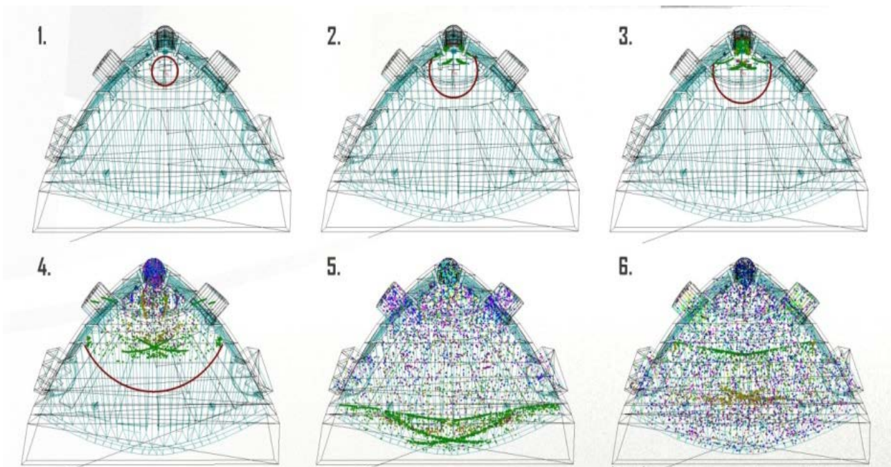
Figure 2: Computer simulation of the Church of the Visitation of Blessed Saint Mary in Poznań developed under the supervision of A. Sygulska, with students: T. Czerniak and A. Czarny-Kropiwnicki.
